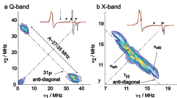
Figure 2. Representative HYSCORE spectra at a) Q-band and b) X-band showing couplings from two ^{31}\text{P} nuclei and the closest olefinic protons, respectively. Insets: FID-detected EPR spectra used to obtain the g -values and Ru hyperfine couplings; experiment (black), simulation (red). The vertical line marks the field position of the HYSCORE measurement, and * marks features from decay product and background resonator signals.
